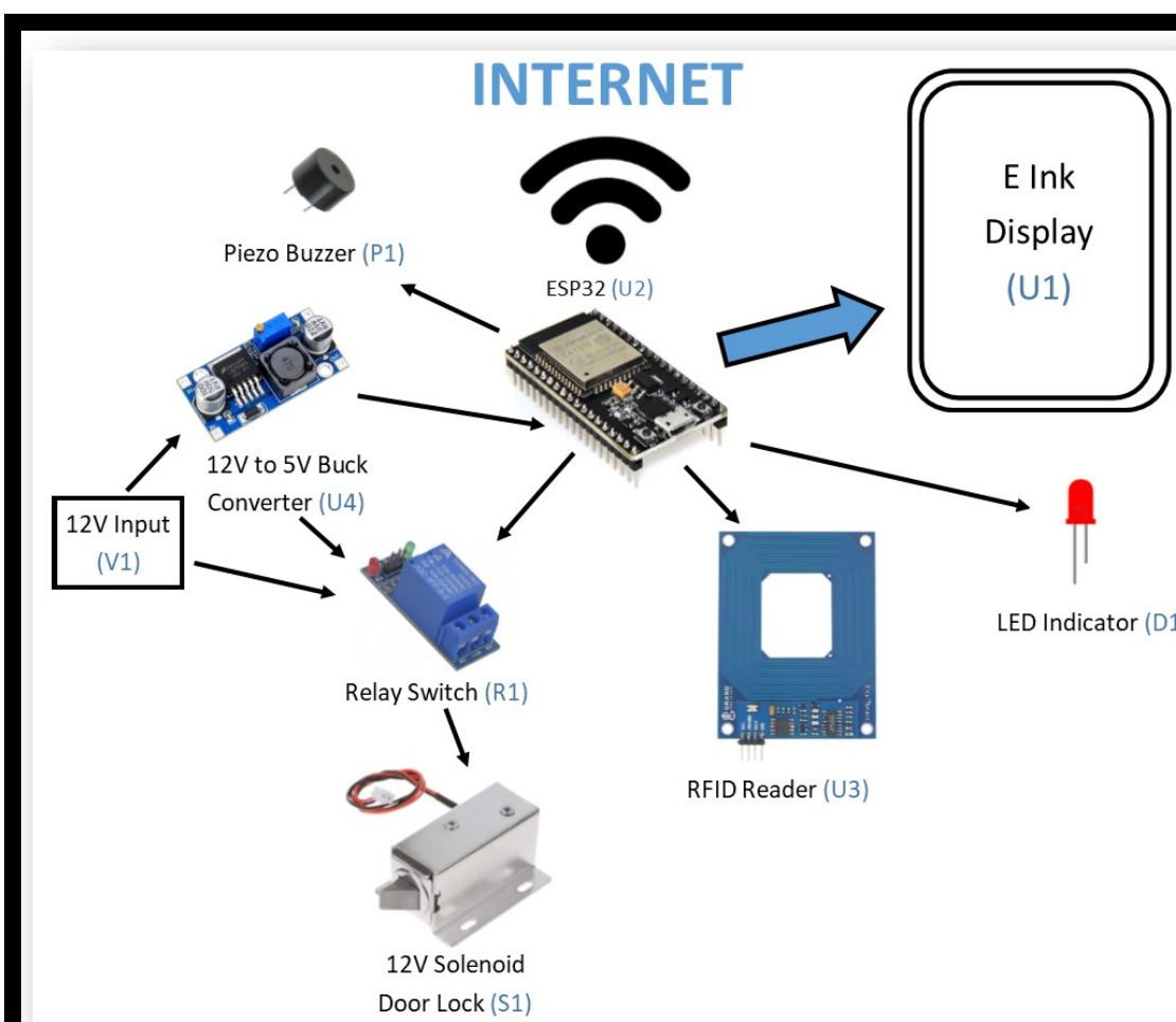
Terminal Block Diagram
